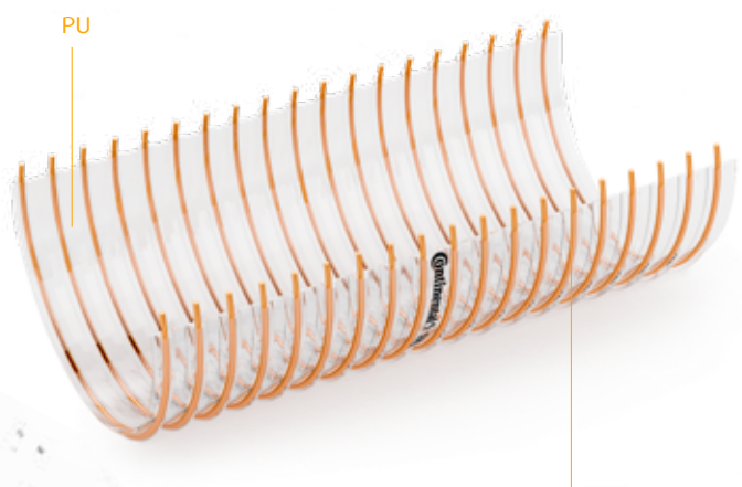
Spirale in acciaio ramato ricoperta in PU PU coated copper-plated steel spiral
